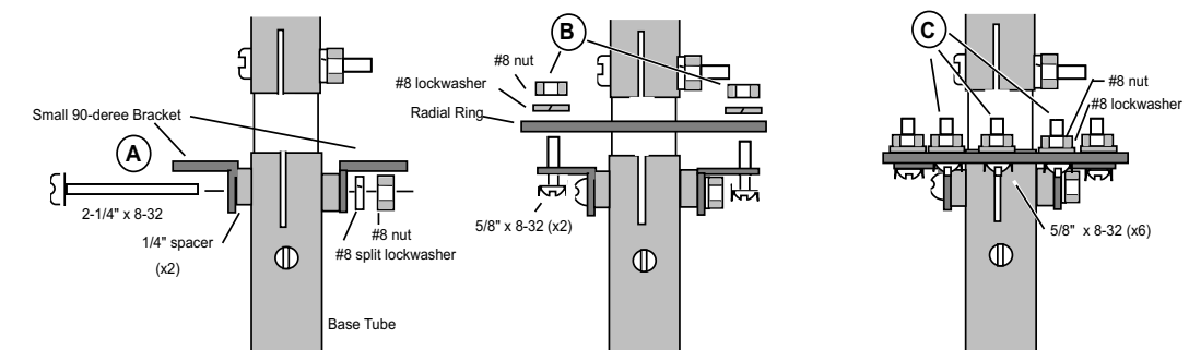
Figure-2: Ground Radial Ring Assembly
